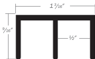
Upper Slide Track or Vertical Upright GS7321
