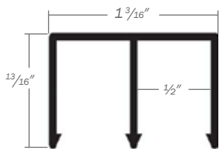
Deep Header Slide Track A54-0372
