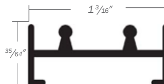
Lower Security Track A54-0371
